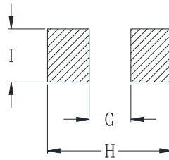
Suggested PWB Layout
